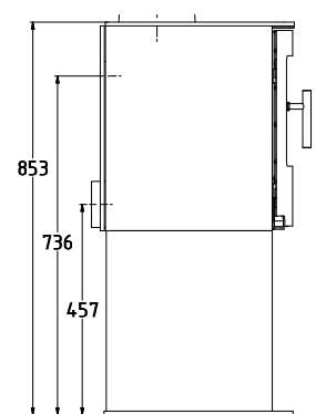
WESTFIRE.TWO / PEDESTAL WEIGHT: 135 KG
